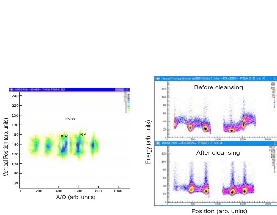
Figure 1: The two dimensional spectrum of the focal plane of the RMS with “holes” is on the left. Energy vs position spectra (taken with the Enge spectrometer) are on the right. Note the non-uniform energy gains as a function of position. Cleansing the wires can make these planes useable again.
